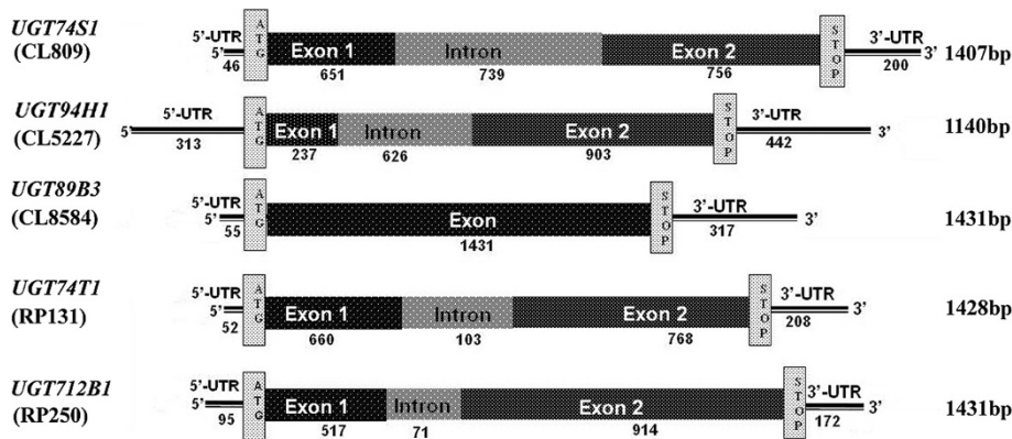
Figure 2 Structural organization of the five flax UGT genes belonging to five sub-families. Exons, introns and UTRs are illustrated with their respective length (bp) indicated below each region. The total length of the coding regions is shown on the right.
