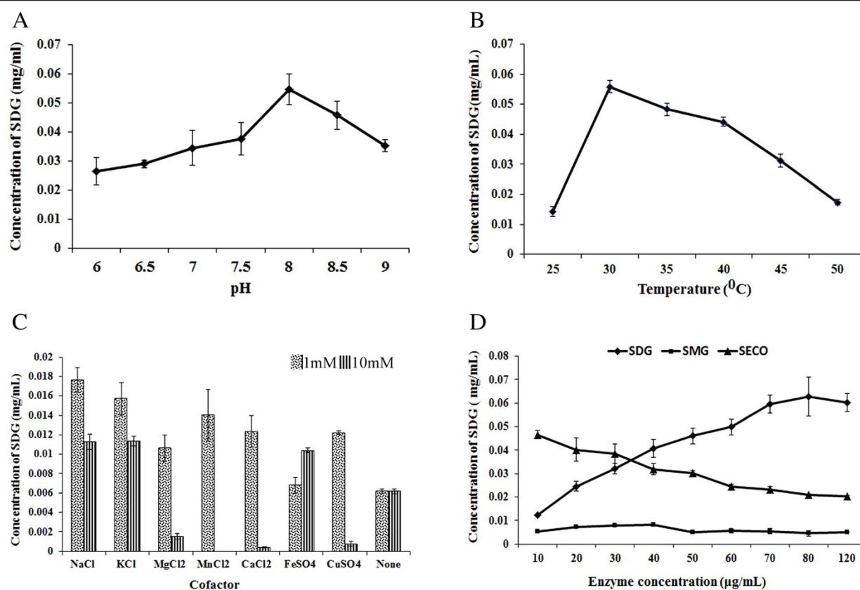
Figure 11 Optimization of UGT74S1 reaction conditions. A , Effect of pH; B , Effect of temperature; C , Effect of two concentrations of seven different metal cofactors; D , Effect of enzyme concentration.
