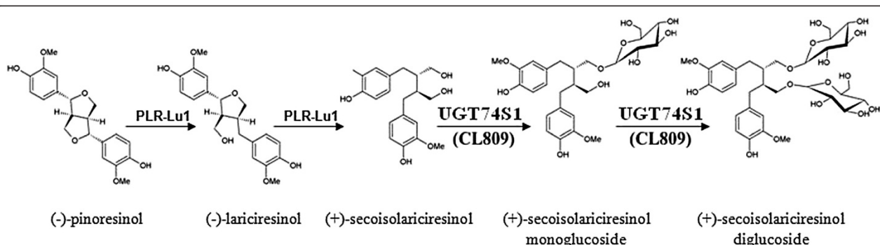
Figure 12 Proposed model for secoisolariciresinol diglucoside (SDG) lignan biosynthesis in flax plants. Secoisolariciresinol (SECO) undergoes sequential glucosylations by UGT74S1 that catalyzes both the first glucosylation of SECO to form secoisolariciresinol monoglucoside (SMG) and the second glucosylation of SMG to SDG.
