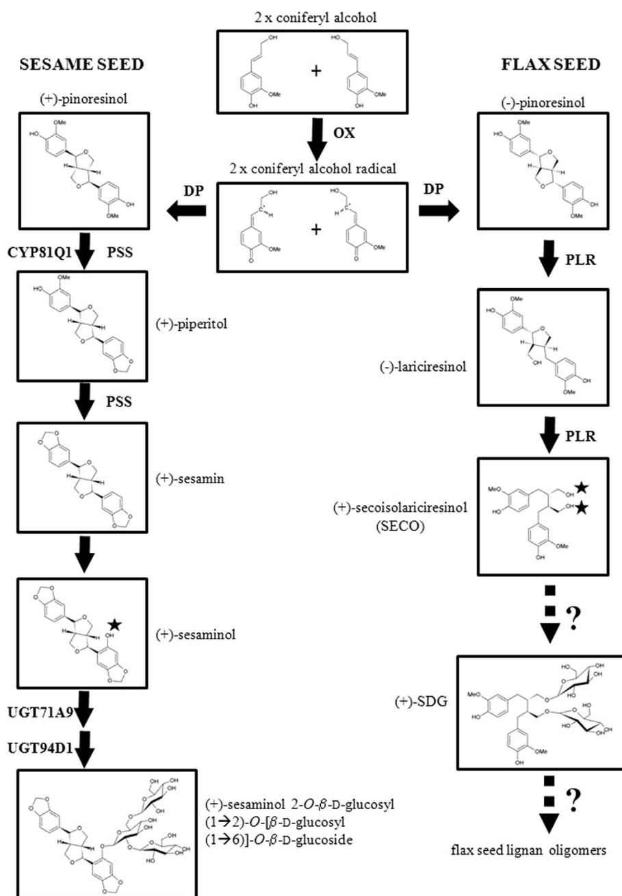
Figure 1 Lignan biosynthesis pathways in sesame and flax starting from coniferyl alcohol. OX, oxidation; DP, dirigent protein; PLR, pinoresinol-lariciresinol reductase; PSS, piperitol sesamin synthase; SDG, secoisolariciresinol diglucoside. Stars indicate the hydroxyl groups glycosylated in sesaminol and secoisolariciresinol. Adapted from Kim et al. [31] with the permission of Dr. Honoo Satake and the PCP editorial office.
