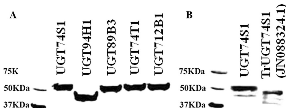
Figure 6 Western blots of His Tag-purified proteins for (A) five UGTs and (B) UGT74S1 and a truncated form encoded by accession number JN088324.1 ( TrUGT74S1 ) [27] using antiXpress™ antibody. M, Western C precision plus protein marker mixed with conjugant (BioRad).
